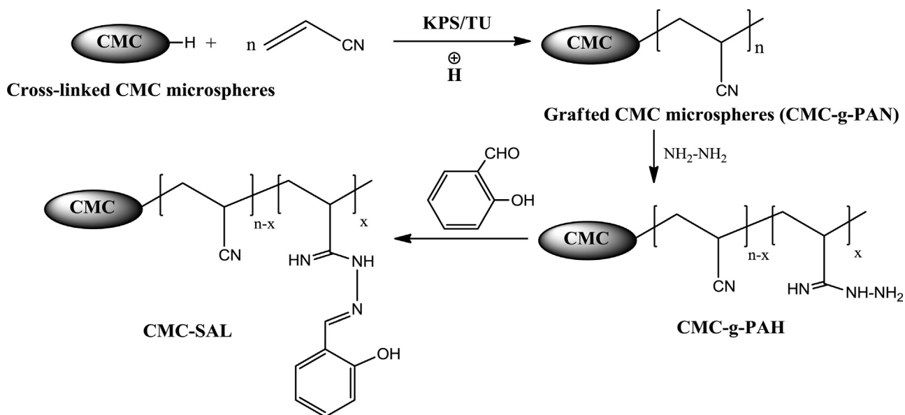
Scheme 1. Synthesis of CMC-SAL chelating microspheres.
