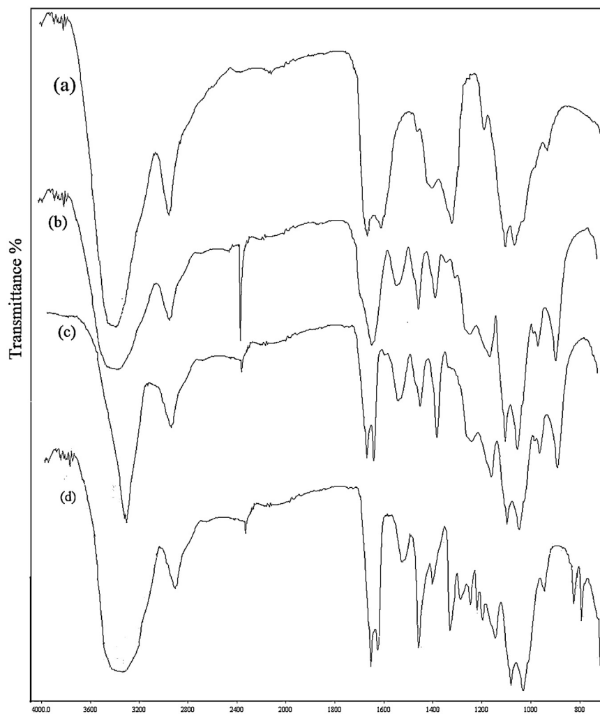
Fig. 1. FTIR spectra of (a) native CMC, (b) CMC-g-PAN, (c) CMC-g-PAH and (d) CMC-SAL.
